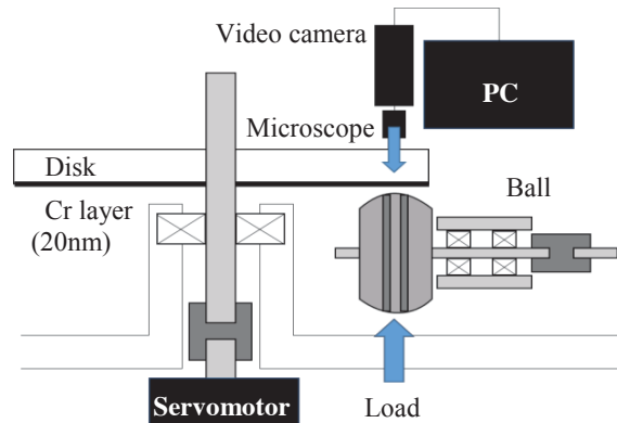
Figure 1 Disk-on-ball friction tester with optical interferometry.
