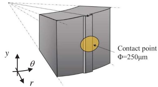
Figure 4 Analytical model for FEM analysis.
