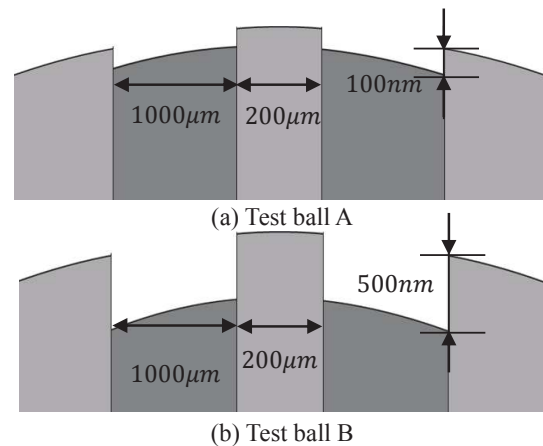
Figure 2 Illustrations of the test balls with downsteps.
