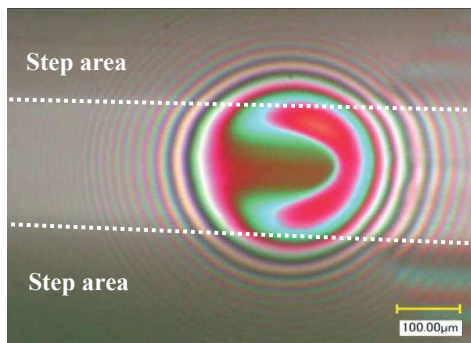
Figure 4 EHL film shape for test ball A at rotational speed of 1.5 m/s.
