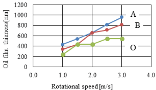
Figure 3 Central EHL film thicknesses at various the rotational speed.
