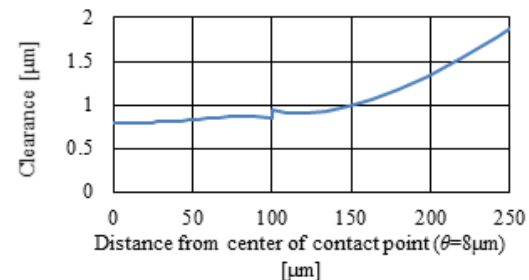
Figure 6 Clearance distribution between disk and ball A calculated from result in Figure 5.
