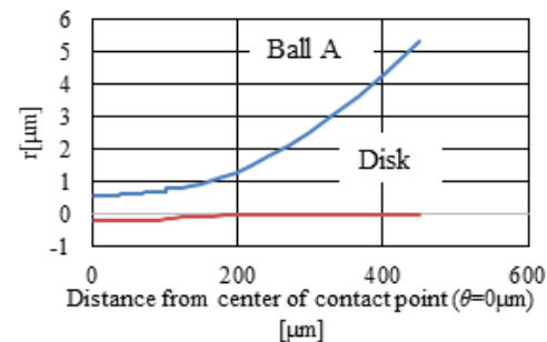
Figure 5 Deformation of disk and ball for pressure distribution calculated using the Reynolds equation.
