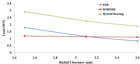
Figure 2 Load carrying capacity by different bearings.
