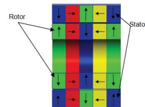
Figure 1 RMD Arrangement.
