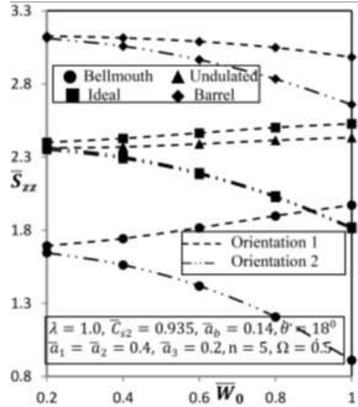
Figure 3 Variation of \bar{S}_{zz} with \bar{W}_0 .
