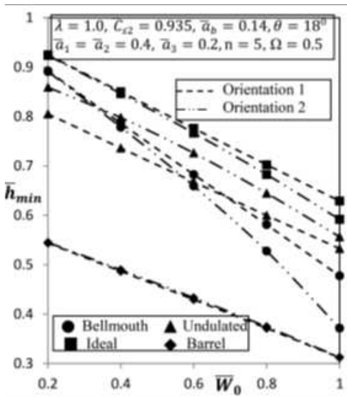
Figure 2 Variation of \bar{h}_{min} with \bar{W}_0 .
