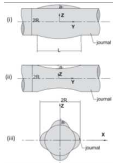
Figure 1 Different geometric irregularities of journal (i) Barrel, (ii) Bellmouth, (iii) Undulations.
