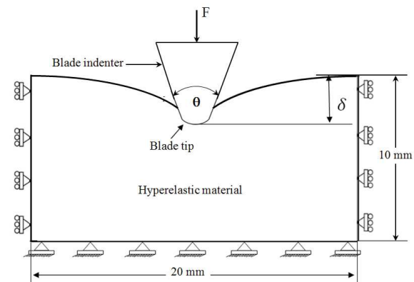
Figure 1 Schematic illustration of the indentation model; a rigid blade indenting a rubber surface.
